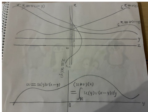
Convolution.
